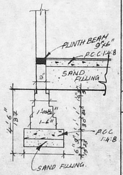
FOUNDATION DETAILS
