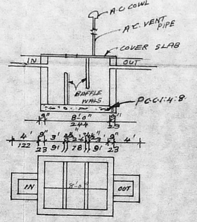
PLAN AND SEC. OF SEPT. TANK
